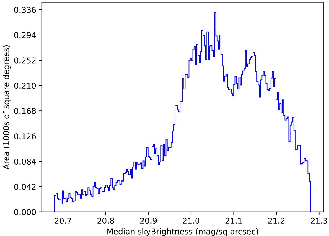
roll_pause_mjdp180_v3.4_10yrs All sky r band: Median skyBrightness
