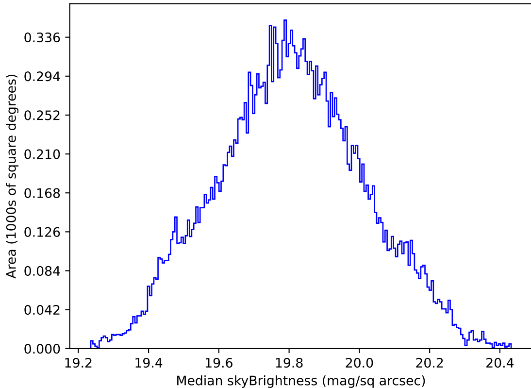
roll_pause_mjdp180_v3.4_10yrs All sky all bands: Median skyBrightness
