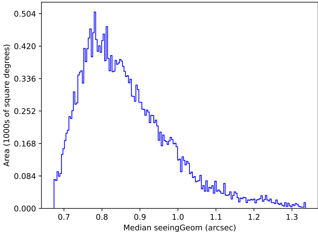
roll_pause_mjdp180_v3.4_10yrs Yr 1 z band: Median seeingGeom
