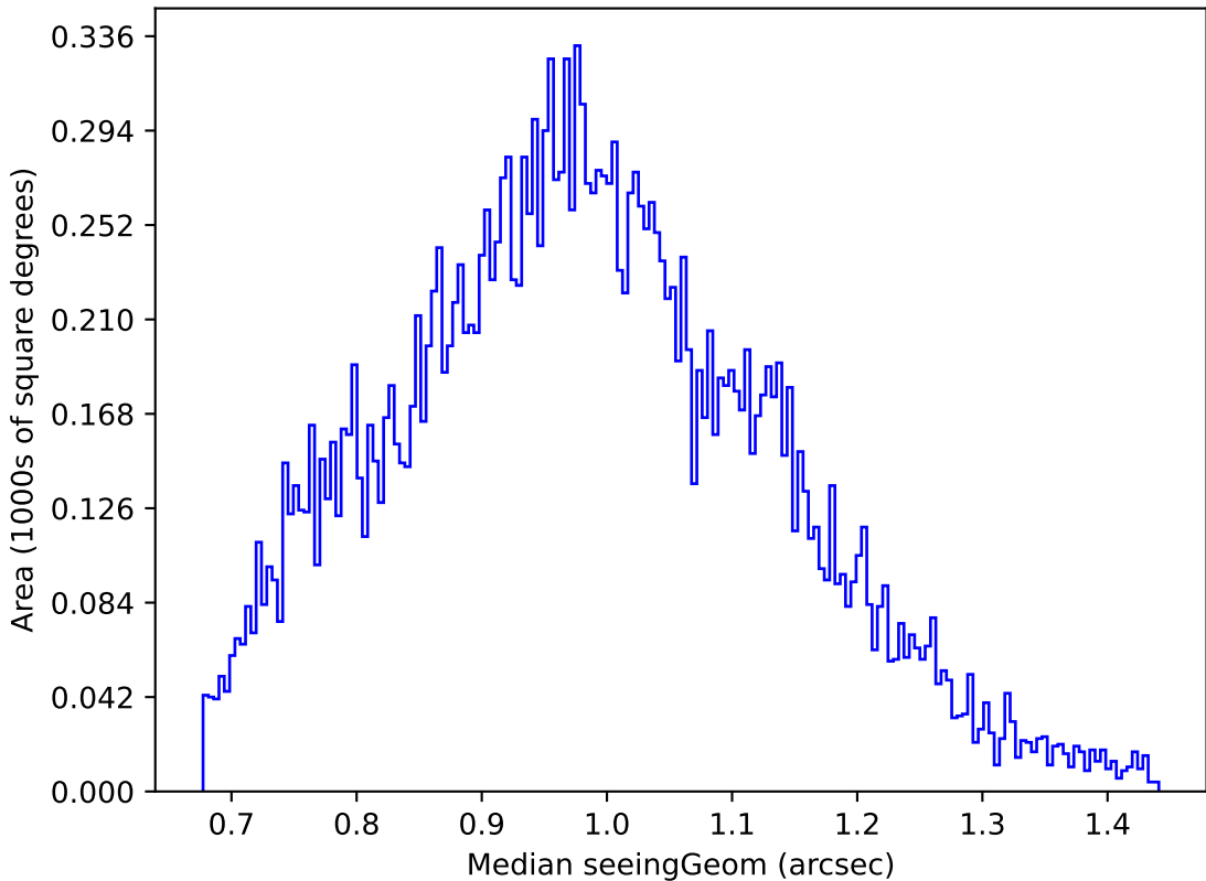
roll_pause_mjdp180_v3.4_10yrs Yr 1 u band: Median seeingGeom
