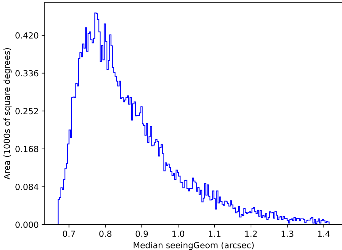
roll_pause_mjdp180_v3.4_10yrs Yr 1 r band: Median seeingGeom
