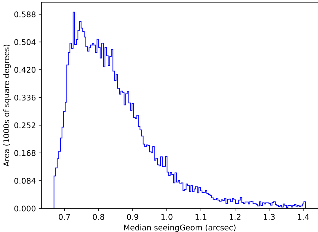
roll_pause_mjdp180_v3.4_10yrs Yr 1 i band: Median seeingGeom
