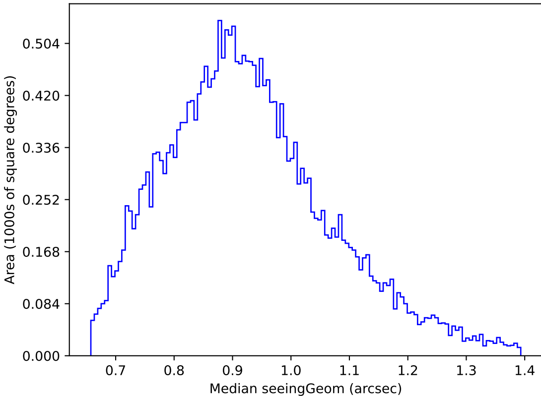
roll_pause_mjdp180_v3.4_10yrs Yr 1 g band: Median seeingGeom
