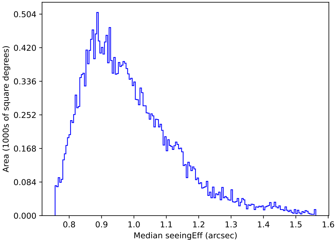
roll_pause_mjdp180_v3.4_10yrs Yr 1 z band: Median seeingEff
