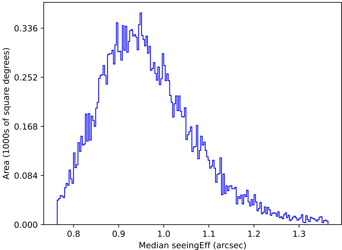
roll_pause_mjdp180_v3.4_10yrs Yr 1 y band: Median seeingEff
