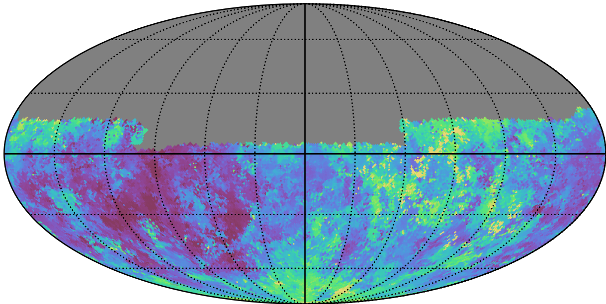
roll_pause_mjdp180_v3.4_10yrs Yr 1 u band: Median seeingEff
