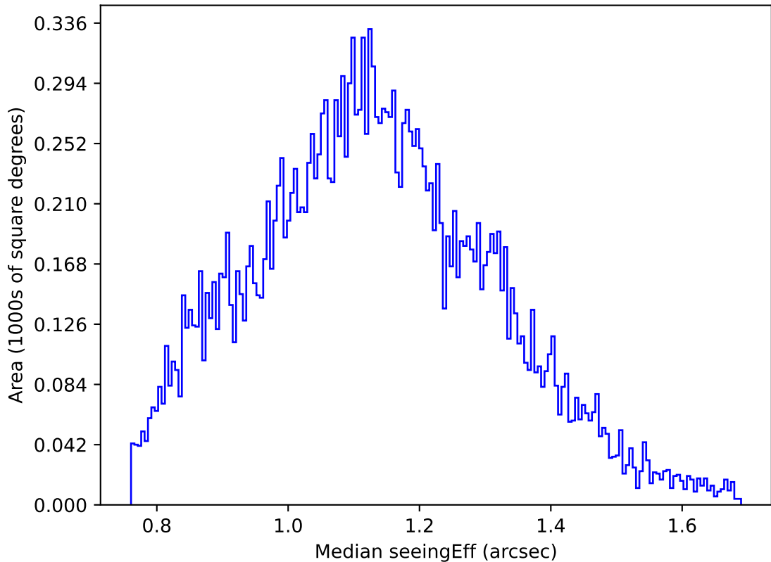
roll_pause_mjdp180_v3.4_10yrs Yr 1 u band: Median seeingEff
