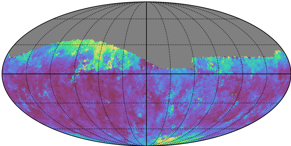
roll_pause_mjdp180_v3.4_10yrs Yr 1 r band: Median seeingEff
