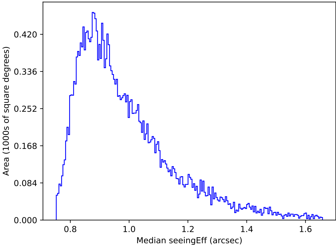
roll_pause_mjdp180_v3.4_10yrs Yr 1 r band: Median seeingEff
