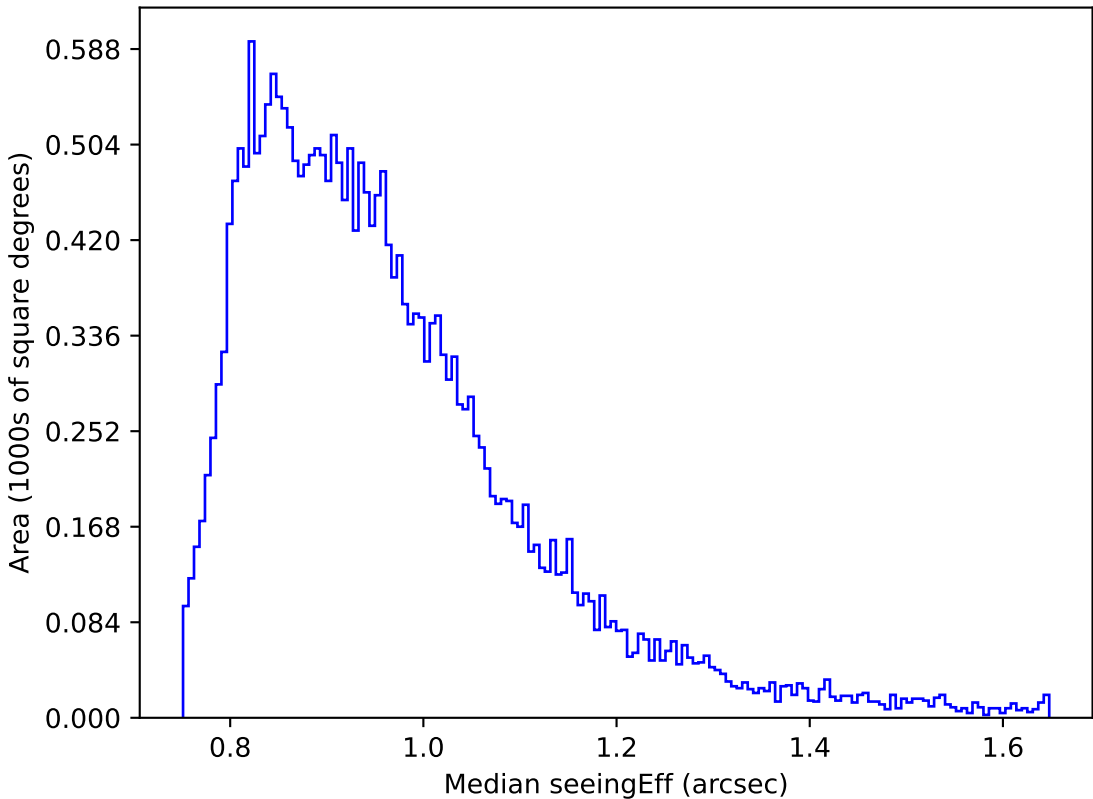
roll_pause_mjdp180_v3.4_10yrs Yr 1 i band: Median seeingEff
