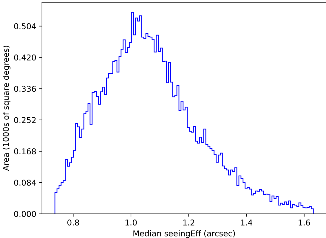
roll_pause_mjdp180_v3.4_10yrs Yr 1 g band: Median seeingEff
