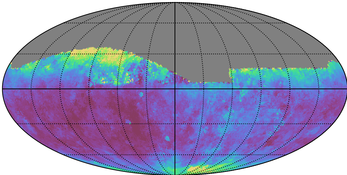
roll_pause_mjdp180_v3.4_10yrs Yr 1 all bands: Median seeingEff
