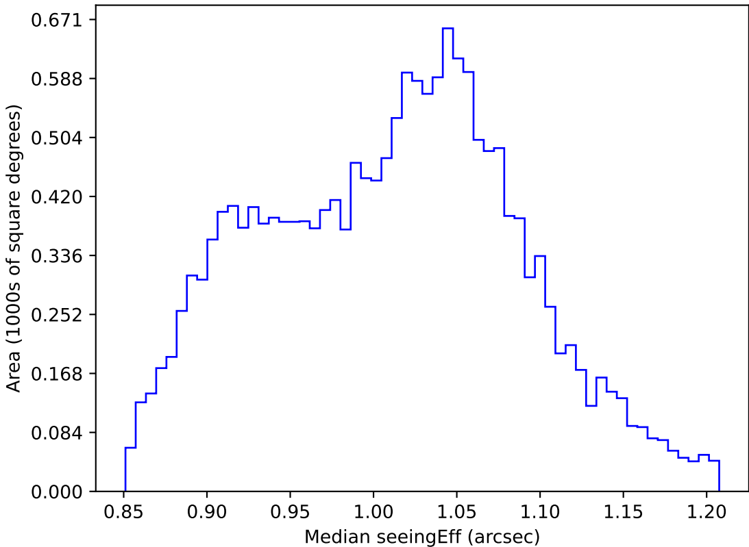
roll_pause_mjdp180_v3.4_10yrs WFD z band: Median seeingEff
