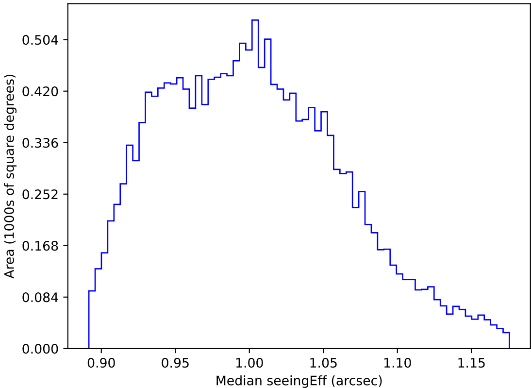
roll_pause_mjdp180_v3.4_10yrs WFD y band: Median seeingEff
