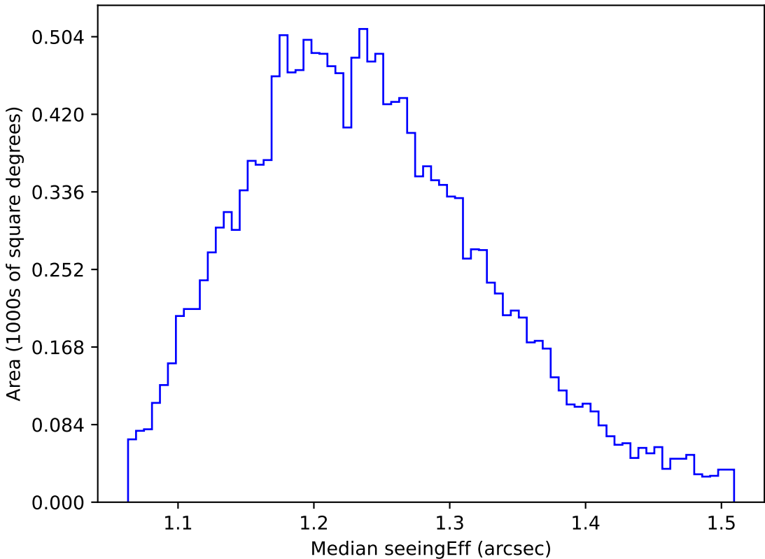
roll_pause_mjdp180_v3.4_10yrs WFD u band: Median seeingEff
