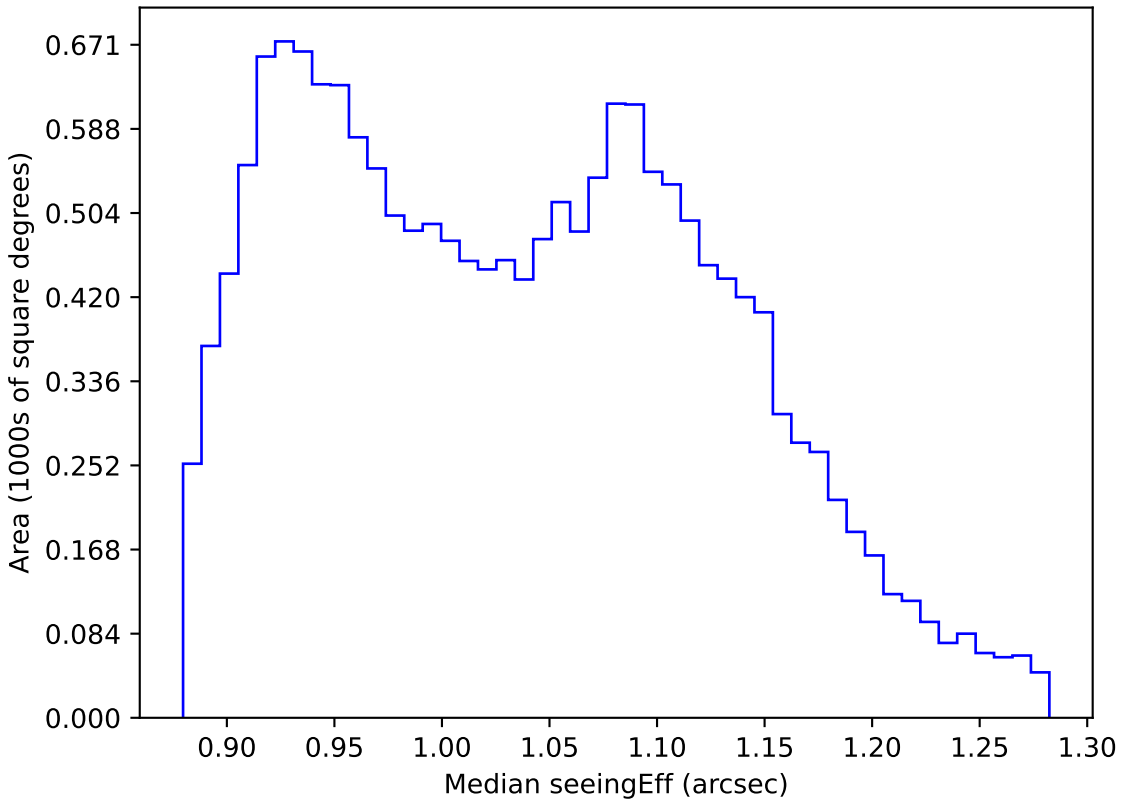
roll_pause_mjdp180_v3.4_10yrs WFD r band: Median seeingEff
