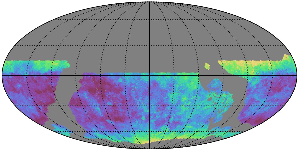
roll_pause_mjdp180_v3.4_10yrs WFD g band: Median seeingEff
