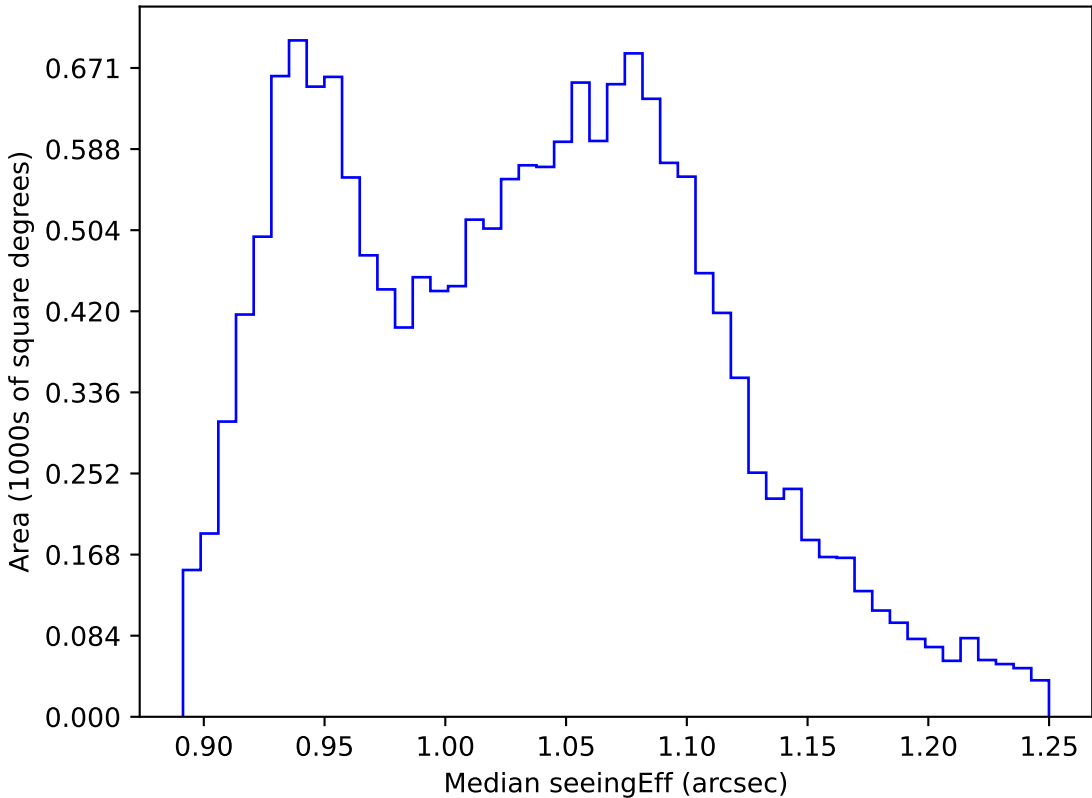
roll_pause_mjdp180_v3.4_10yrs WFD all bands: Median seeingEff
