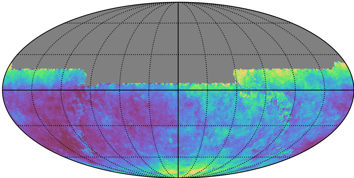
roll_pause_mjdp180_v3.4_10yrs All sky y band: Median seeingEff
