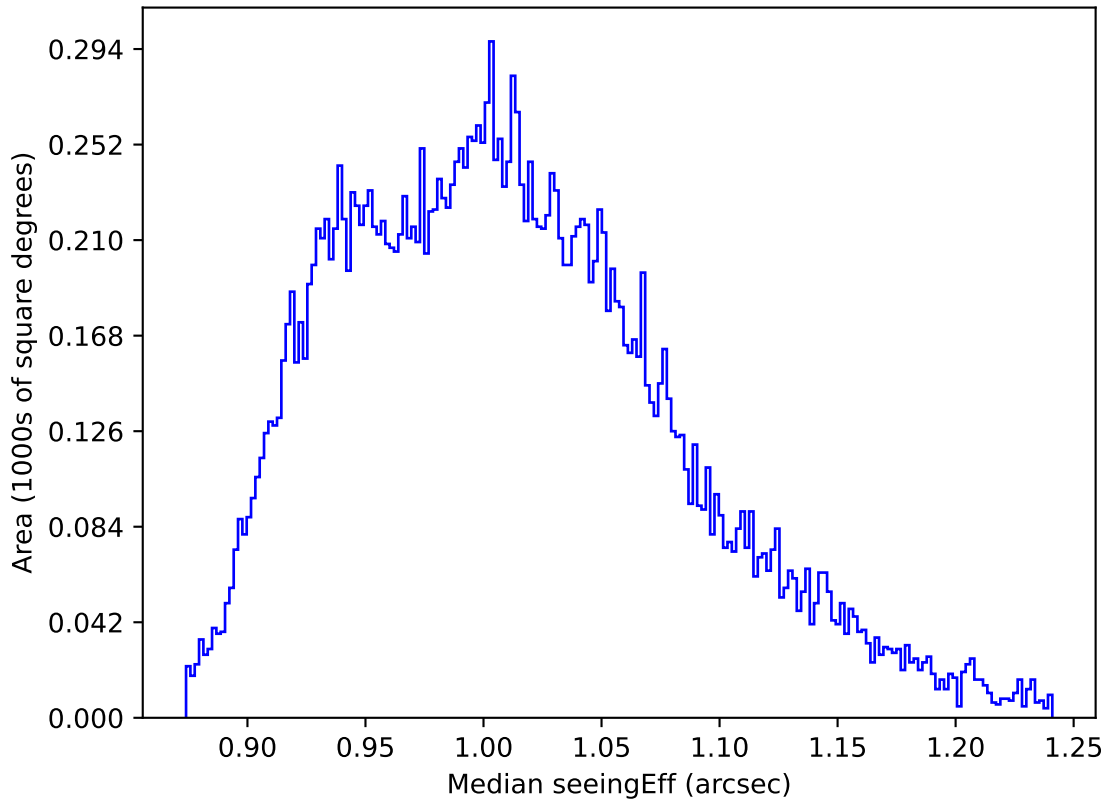
roll_pause_mjdp180_v3.4_10yrs All sky y band: Median seeingEff
