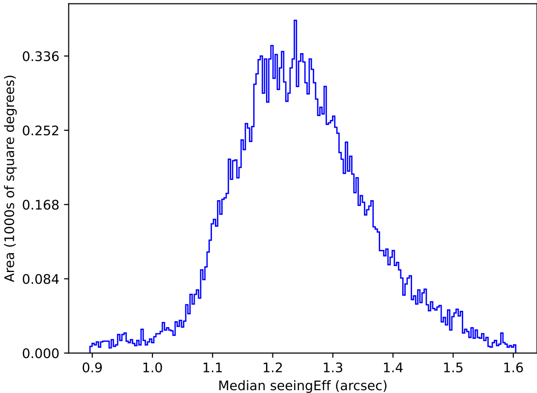
roll_pause_mjdp180_v3.4_10yrs All sky u band: Median seeingEff
