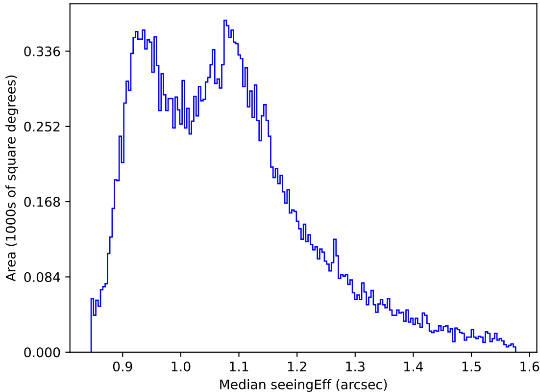
roll_pause_mjdp180_v3.4_10yrs All sky r band: Median seeingEff
