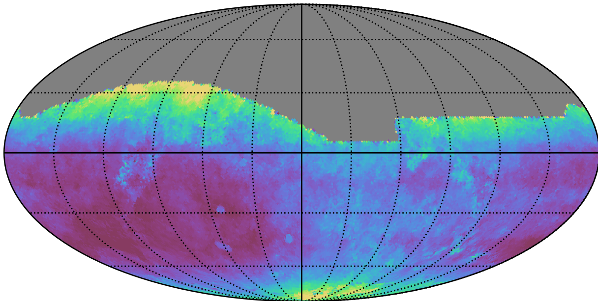
roll_pause_mjdp180_v3.4_10yrs All sky i band: Median seeingEff
