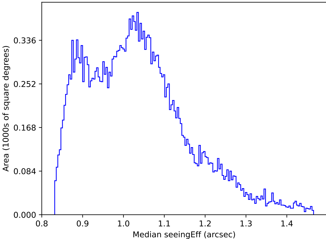
roll_pause_mjdp180_v3.4_10yrs All sky i band: Median seeingEff
