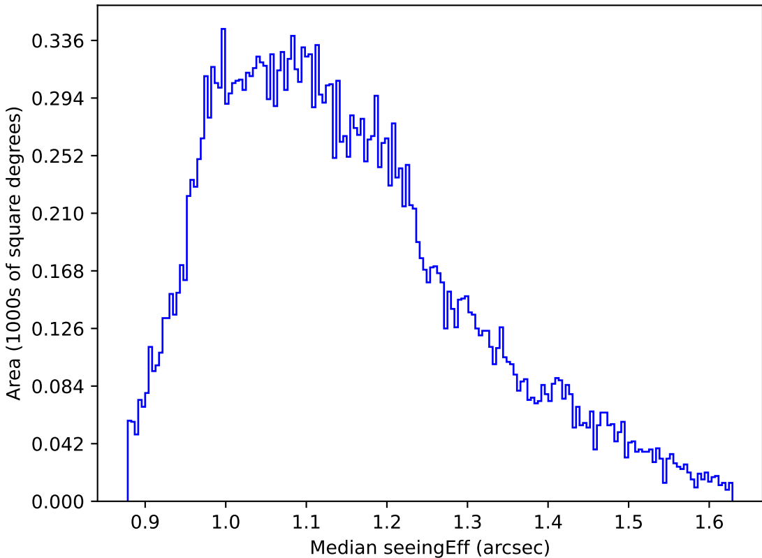
roll_pause_mjdp180_v3.4_10yrs All sky g band: Median seeingEff
