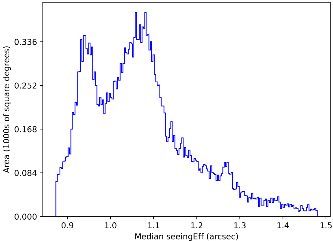
roll_pause_mjdp180_v3.4_10yrs All sky all bands: Median seeingEff
