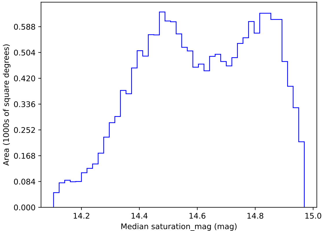
roll_pause_mjdp180_v3.4_10yrs WFD r band: Median saturation_mag
