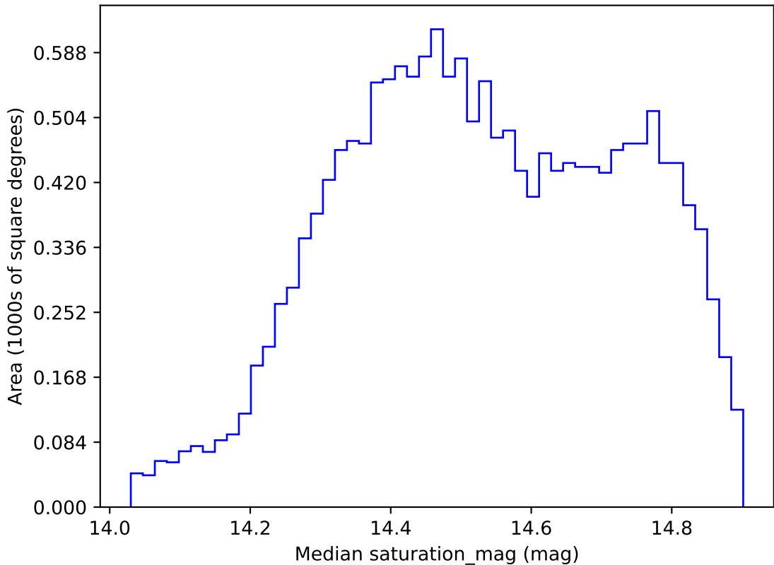
roll_pause_mjdp180_v3.4_10yrs WFD i band: Median saturation_mag
