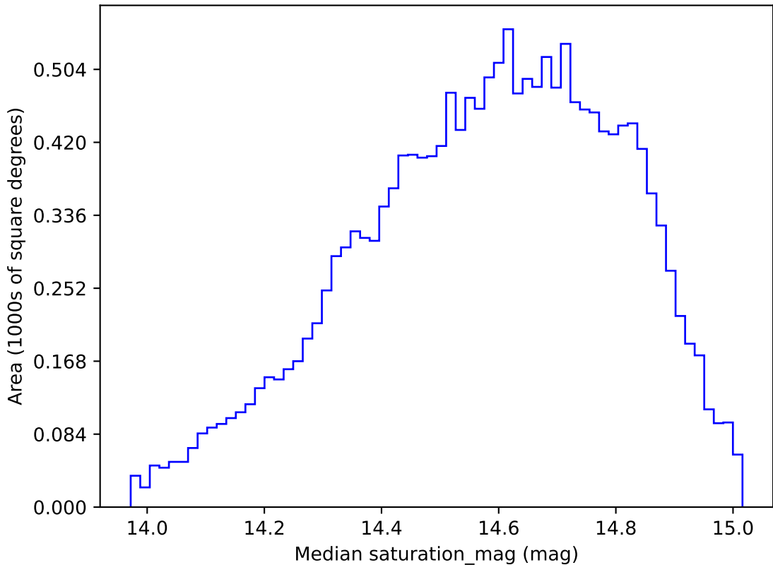
roll_pause_mjdp180_v3.4_10yrs WFD g band: Median saturation_mag
