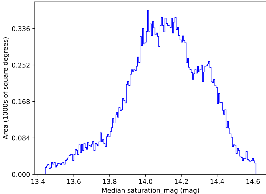
roll_pause_mjdp180_v3.4_10yrs All sky all bands: Median saturation_mag
