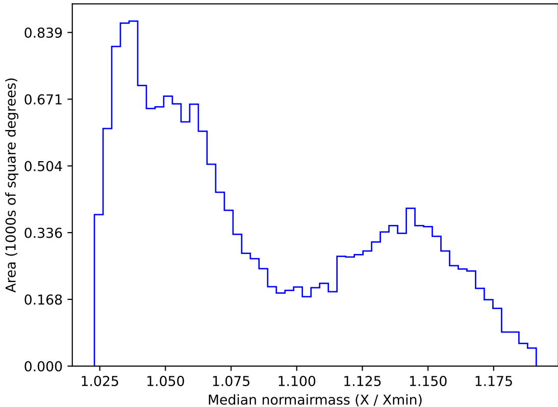
roll_pause_mjdp180_v3.4_10yrs WFD z band: Median normairmass
