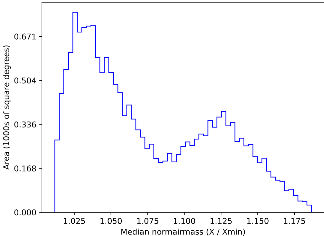
roll_pause_mjdp180_v3.4_10yrs WFD u band: Median normairmass
