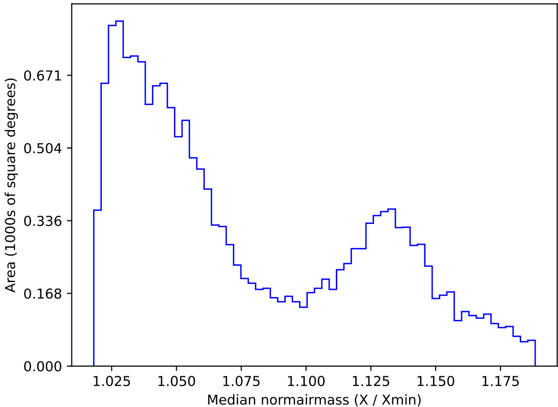
roll_pause_mjdp180_v3.4_10yrs WFD r band: Median normairmass
