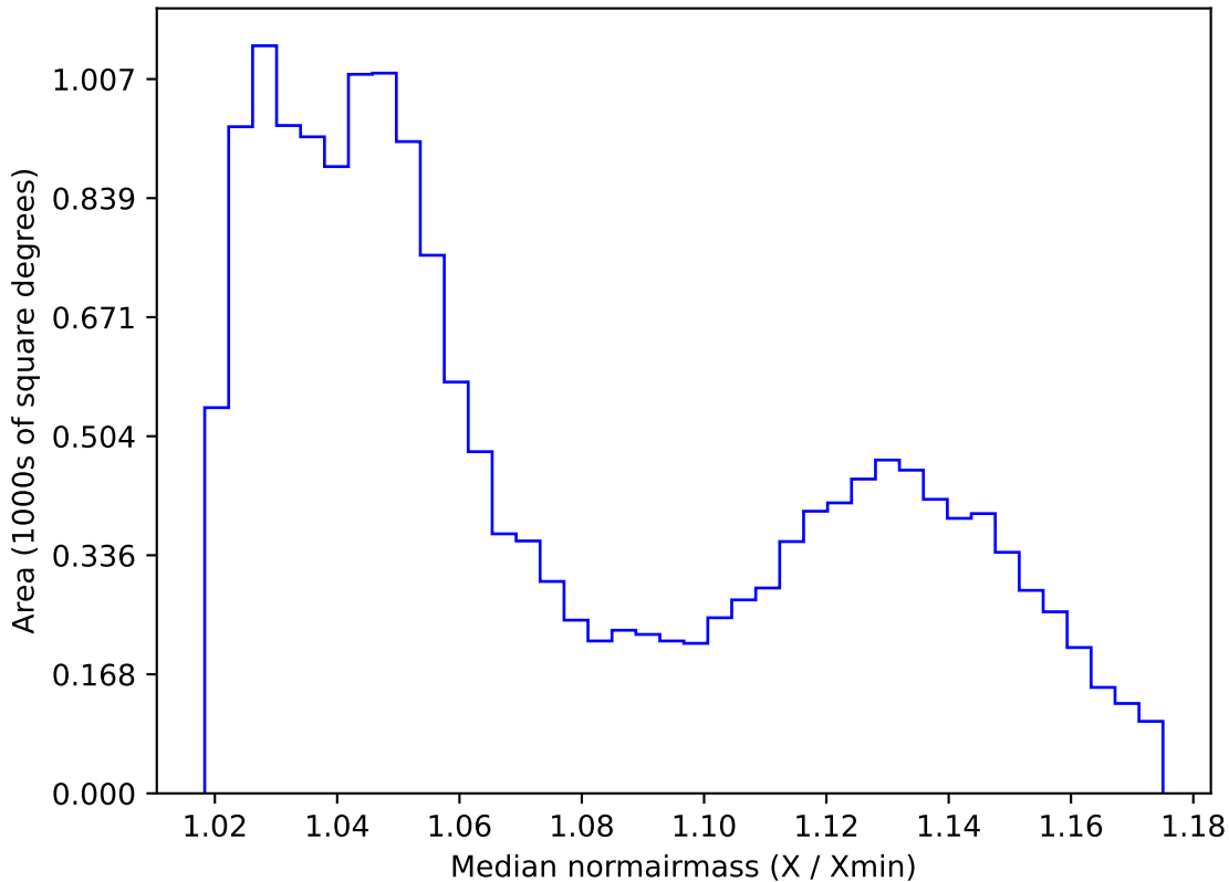
roll_pause_mjdp180_v3.4_10yrs WFD i band: Median normairmass
