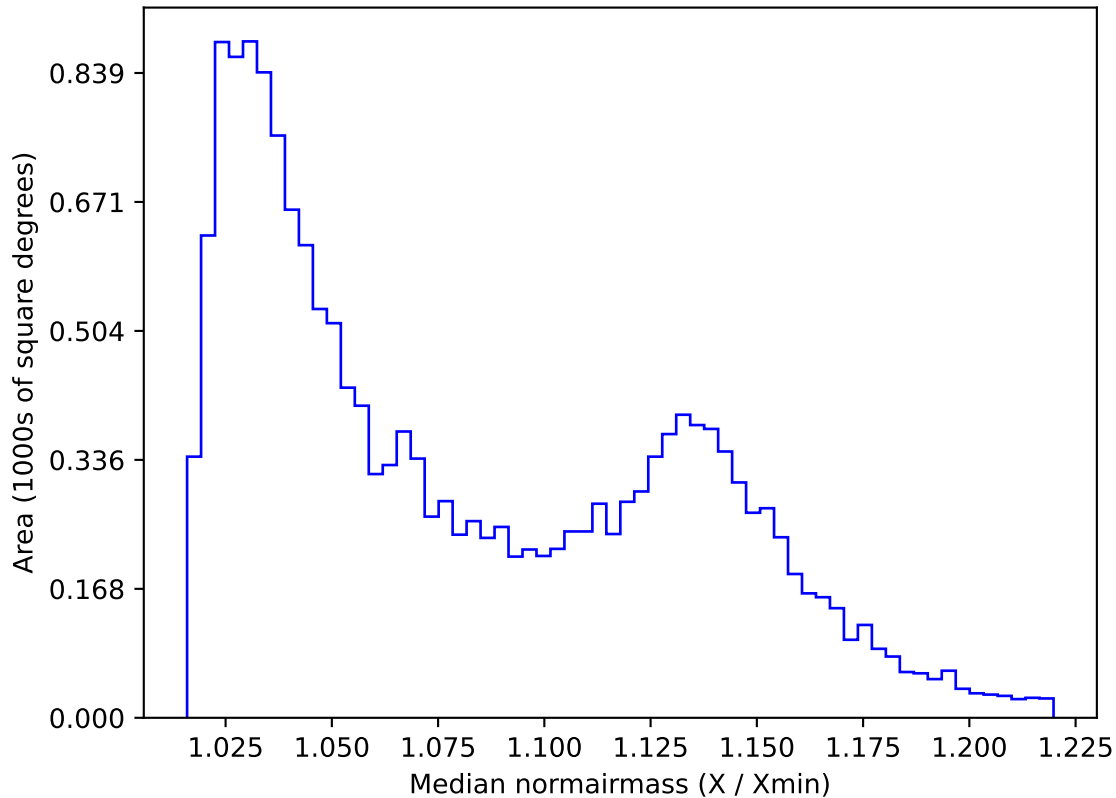
roll_pause_mjdp180_v3.4_10yrs WFD g band: Median normairmass
