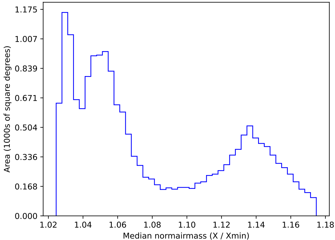
roll_pause_mjdp180_v3.4_10yrs WFD all bands: Median normairmass
