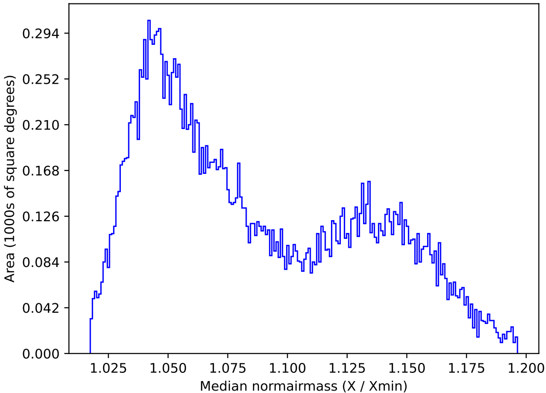
roll_pause_mjdp180_v3.4_10yrs All sky y band: Median normairmass
