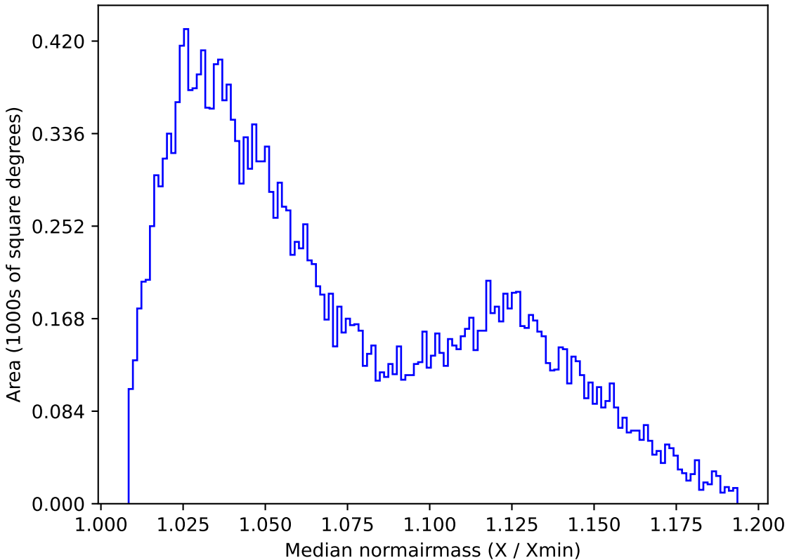
roll_pause_mjdp180_v3.4_10yrs All sky u band: Median normairmass
