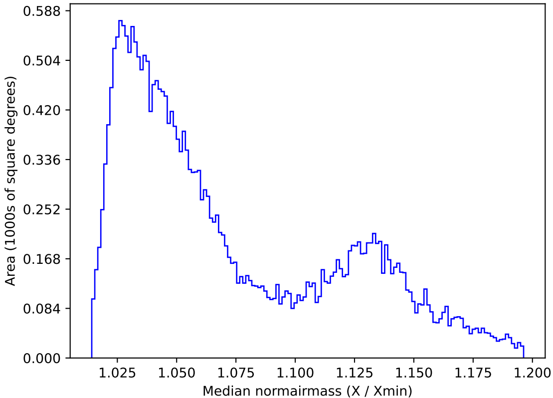
roll_pause_mjdp180_v3.4_10yrs All sky r band: Median normairmass
