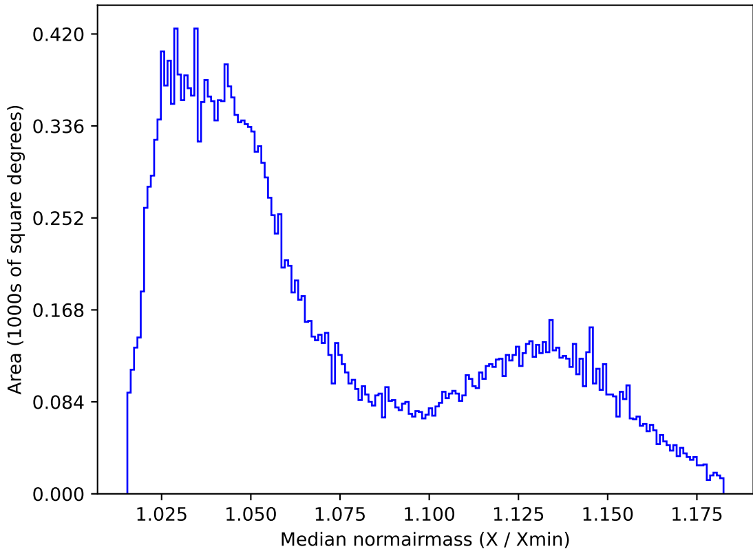
roll_pause_mjdp180_v3.4_10yrs All sky i band: Median normairmass
