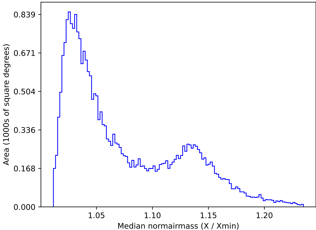
roll_pause_mjdp180_v3.4_10yrs All sky g band: Median normairmass
