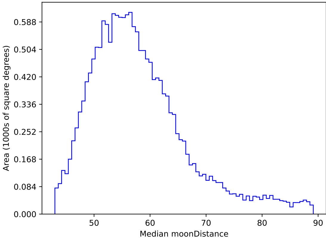
roll_pause_mjdp180_v3.4_10yrs WFD y band: Median moonDistance
