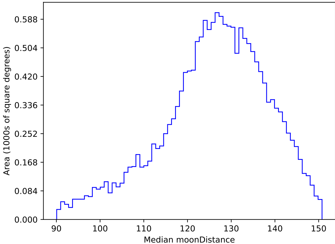
roll_pause_mjdp180_v3.4_10yrs WFD u band: Median moonDistance
