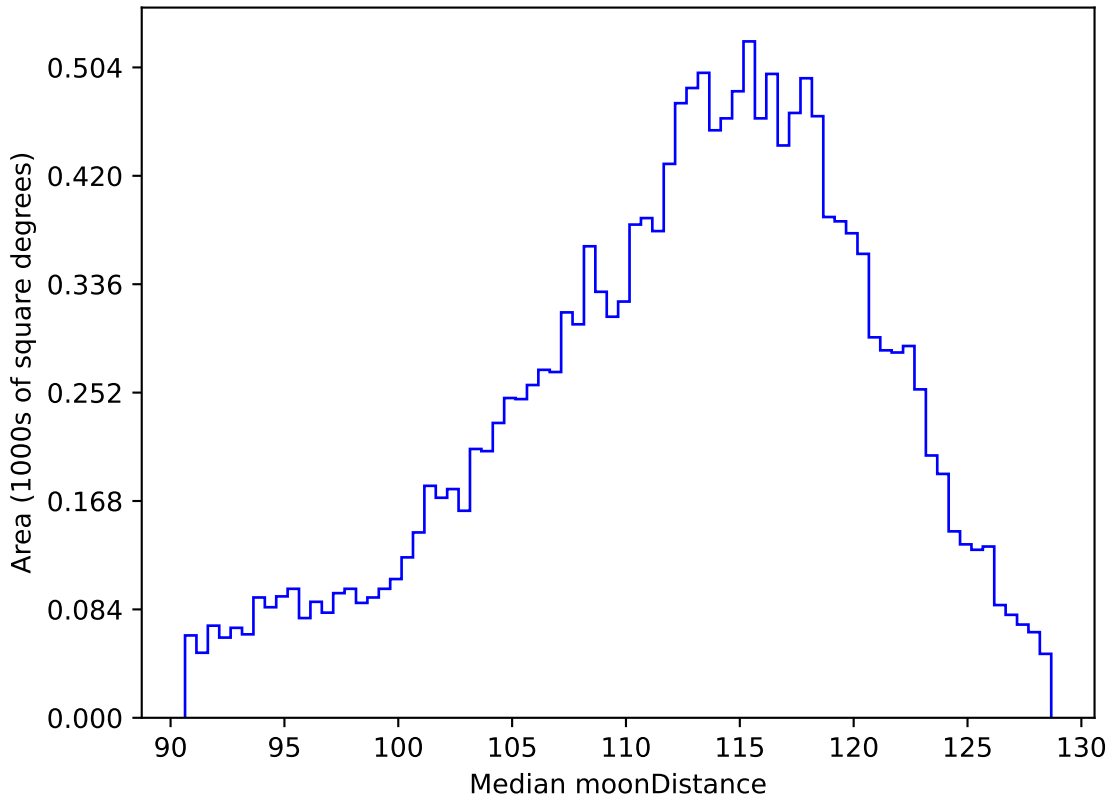
roll_pause_mjdp180_v3.4_10yrs WFD r band: Median moonDistance
