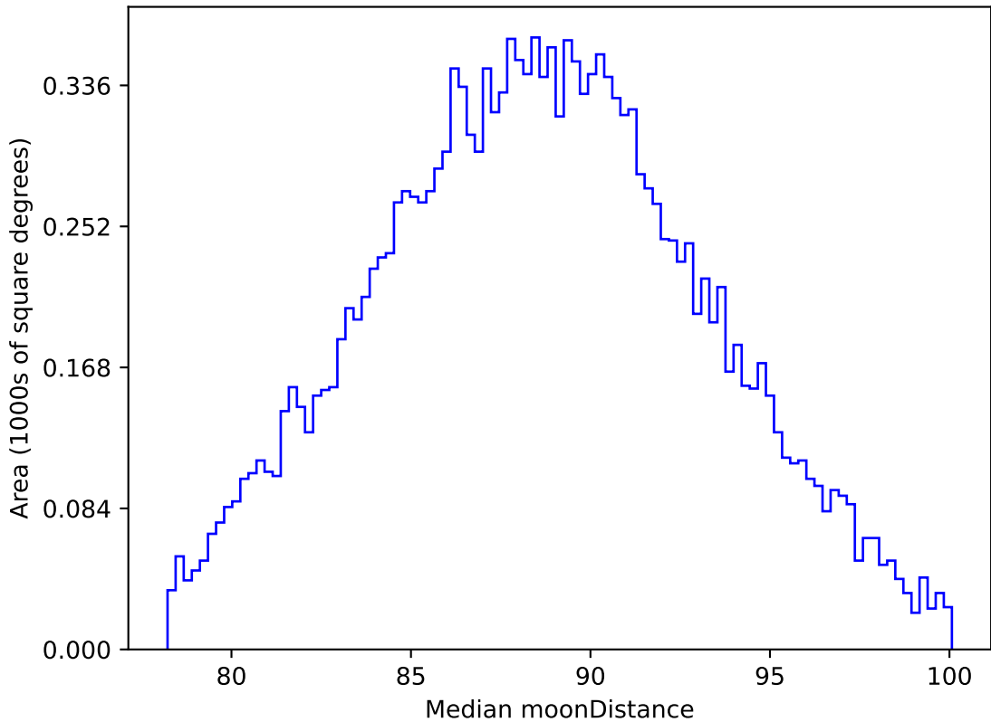
roll_pause_mjdp180_v3.4_10yrs WFD all bands: Median moonDistance
