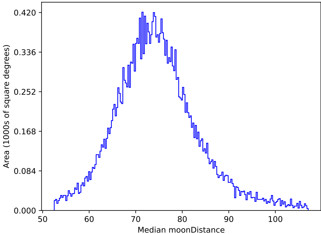
roll_pause_mjdp180_v3.4_10yrs All sky z band: Median moonDistance
